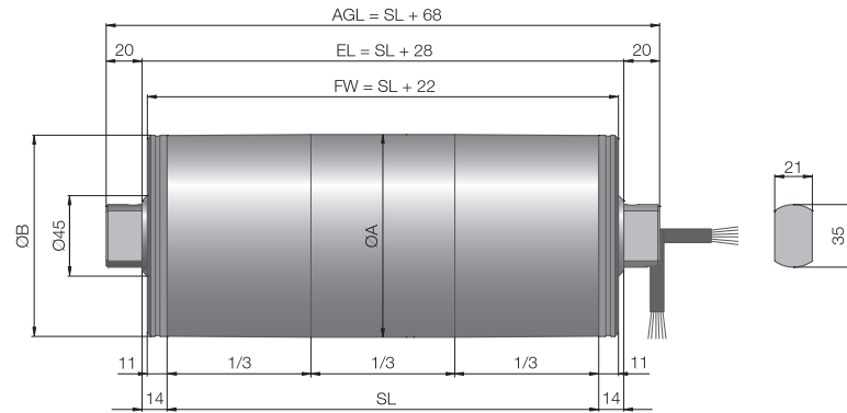
Fig.: Drum motor with shaft cap
