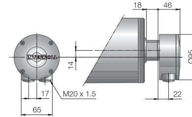
Fig.: Terminal box, aluminium
